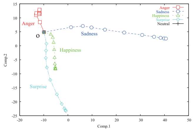
Fig. 10. Virtual emotional space of Proposed Robot B .
